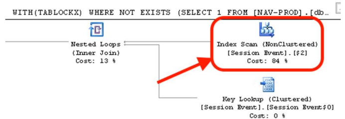
Figure 2 Example of SQL Query Execution Plan Analysis
